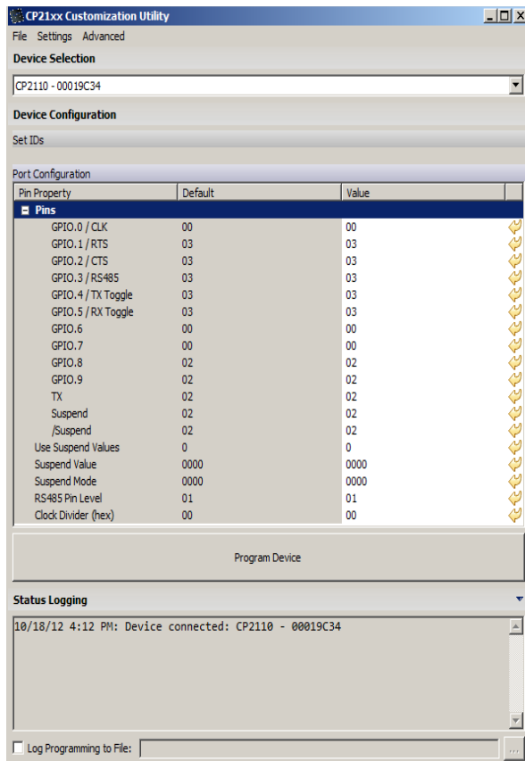
Figure 5. CP2110 (LEFT) and CP2114 (RIGHT) Port Configuration Settings
