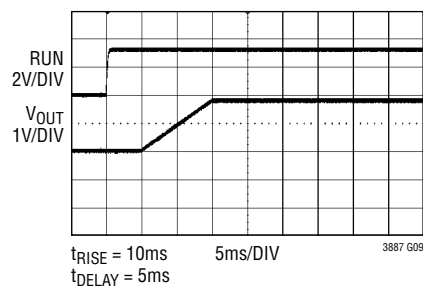
Soft-Start Ramp
