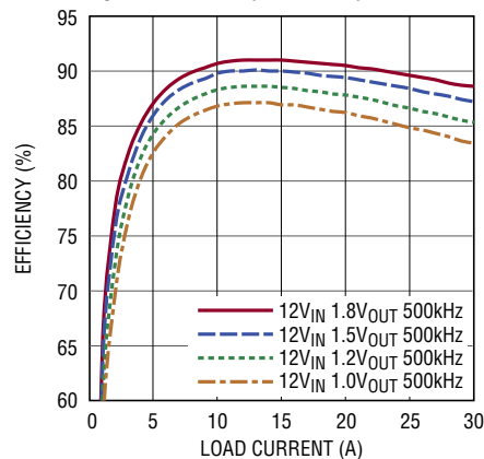
Efficiency vs Load Current F_{SW} = 500\text{kHz} (LTC3887)
