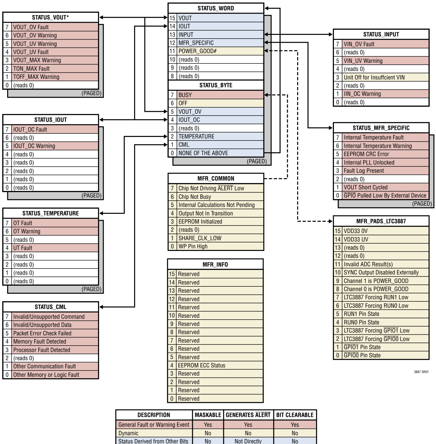
Figure 43. Summary of the Status Registers
