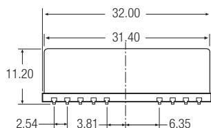
24 PIN SMD Package
