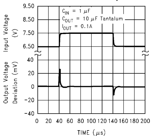
LM1117-5.0 Line Transient Response
