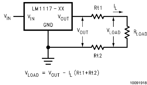
FIGURE 2. Typical Application using Fixed Output Regulator
