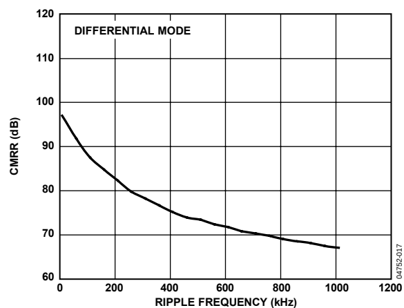
Figure 13. CMRR vs. Ripple Frequency with V_{DD} = 5\text{ V} and 3\text{ V}
