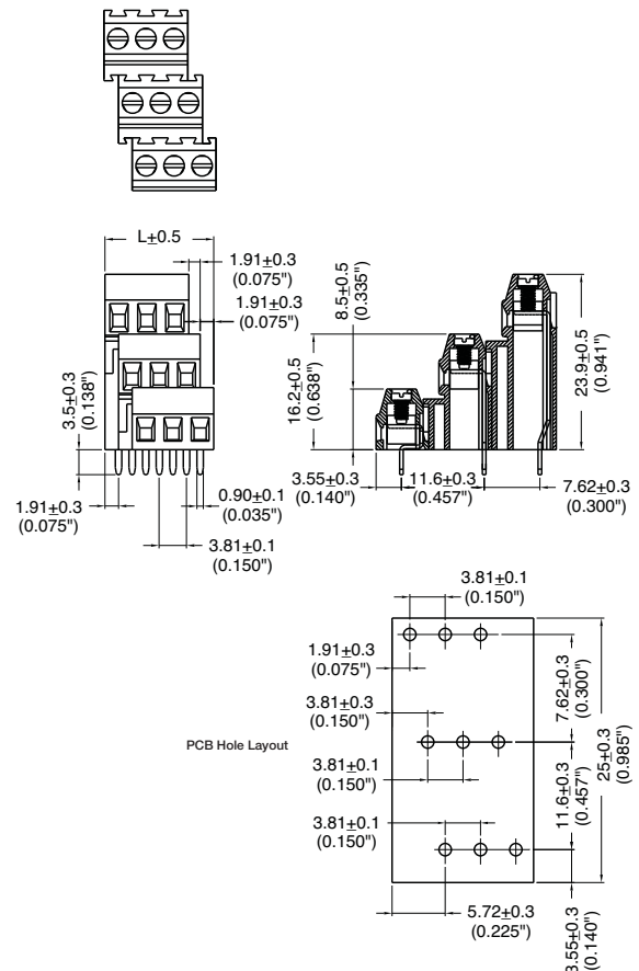
Dimensions - mm (in)
