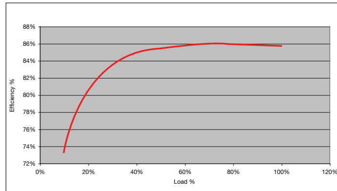
Figure 8 MFA350PS12 @ 230 VAC
