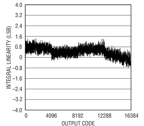
Integral Linearity End Point Fit for CH0 with Internal 2.5V Reference for Differential Input Signals
