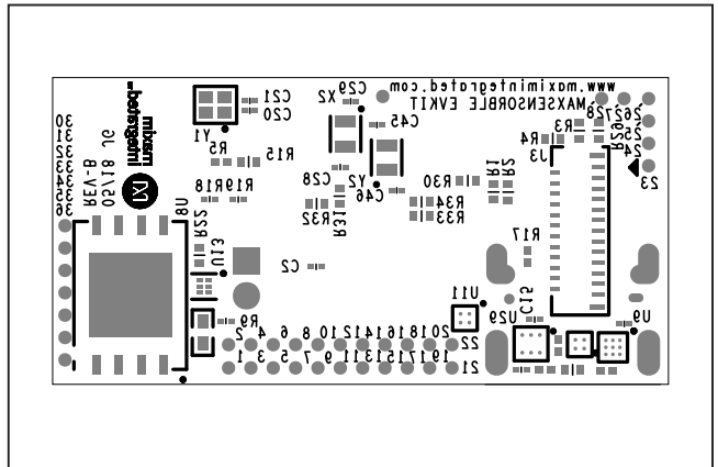
MAXSensorBLE_EVKIT—SILK_BOT
