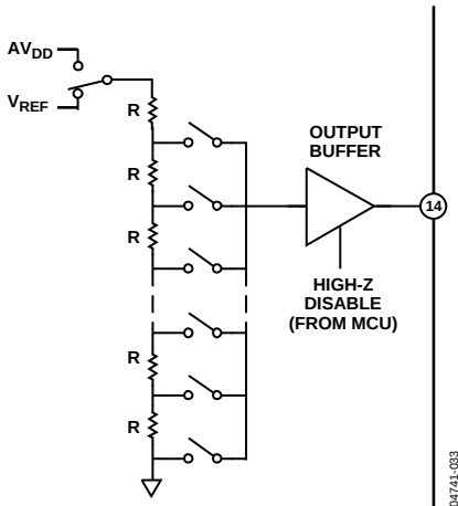
Figure 33. Resistor String DAC Functional Equivalent
