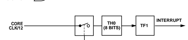
Figure 55. Timer/Counter 0, Mode 3
