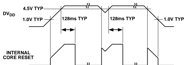
Figure 67. 5 V Part POR Operation
