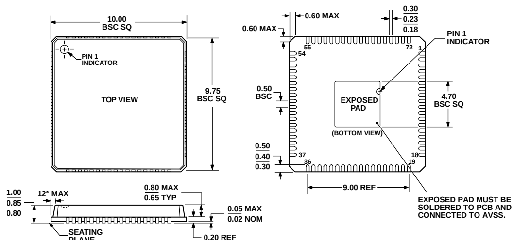
Figure 44. 72-Lead Lead Frame Chip Scale Package [LFCSP_VQ]
