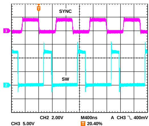
Figure 28. Synchronized to 1 MHz 180° Out of Phase
