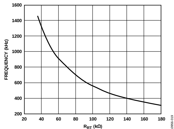
Figure 29. Frequency ( f_{SW} ) vs. R_{RT} Resistor
