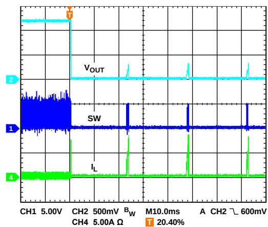
Figure 24. Output Short
