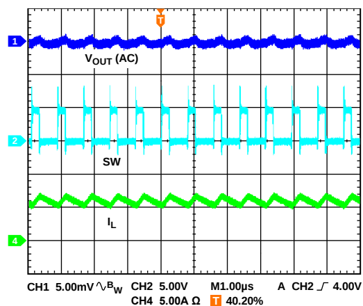
Figure 23. Steady Waveform
