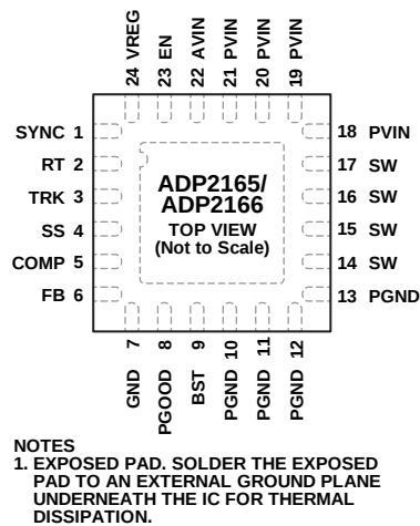
Figure 4. Pin Configuration
