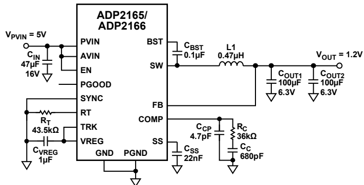
Figure 36. Fixed Output 1.2 V, 5 A/6 A, 1.2 MHz Step-Down Regulator Application
