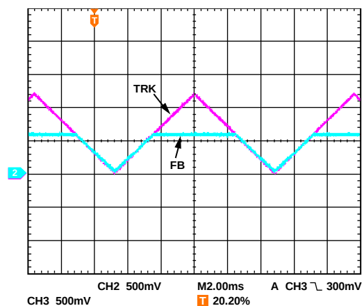
Figure 26. Tracing Function
