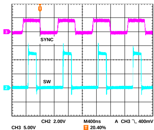
Figure 25. Synchronized to 1 MHz in Phase
