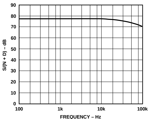
Figure 8. Signal/(Noise and Distortion) vs. Frequency
