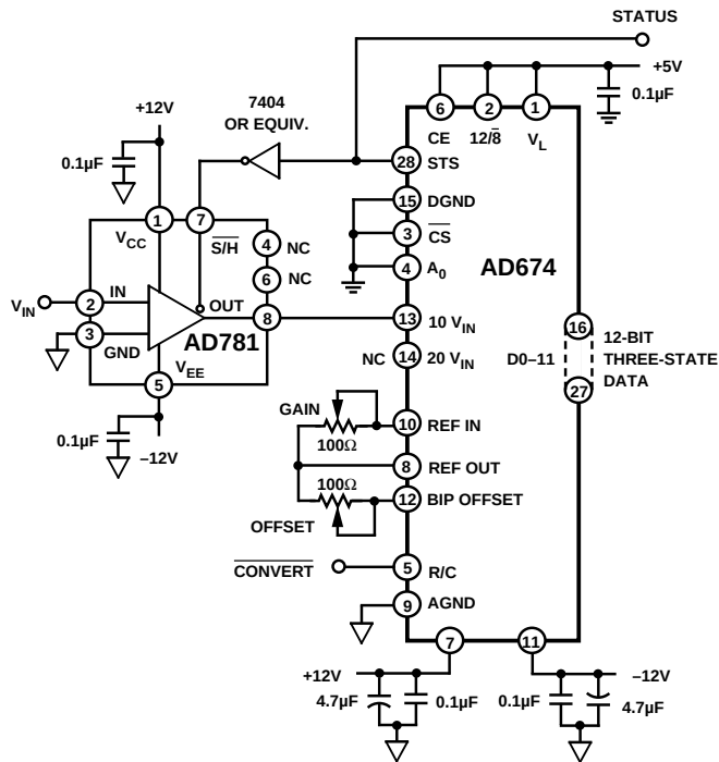
Figure 9. AD781 to AD674 Interface
