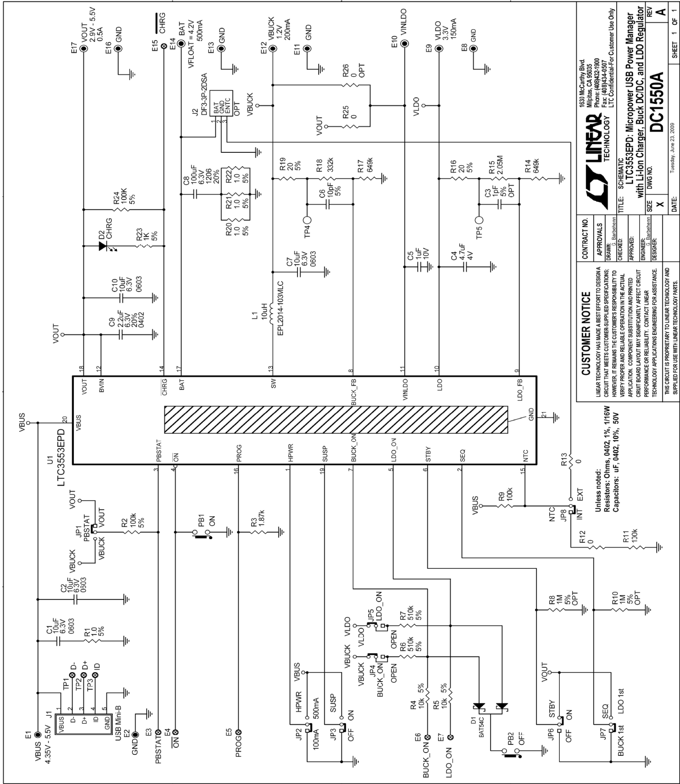
Figure 3. Circuit Schematic
