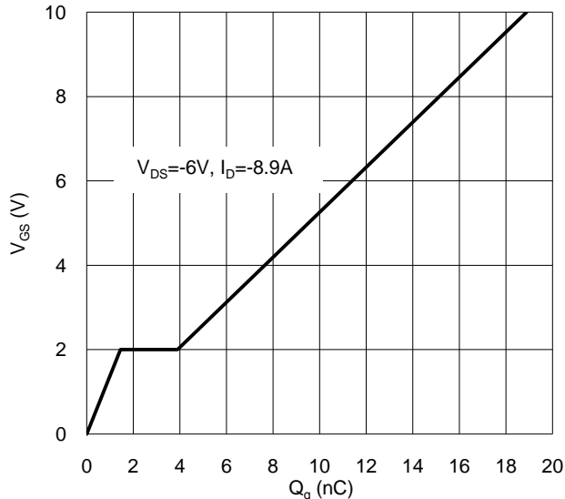
Figure 23. Gate Charge
