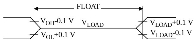
Figure 24. Float Waveforms
