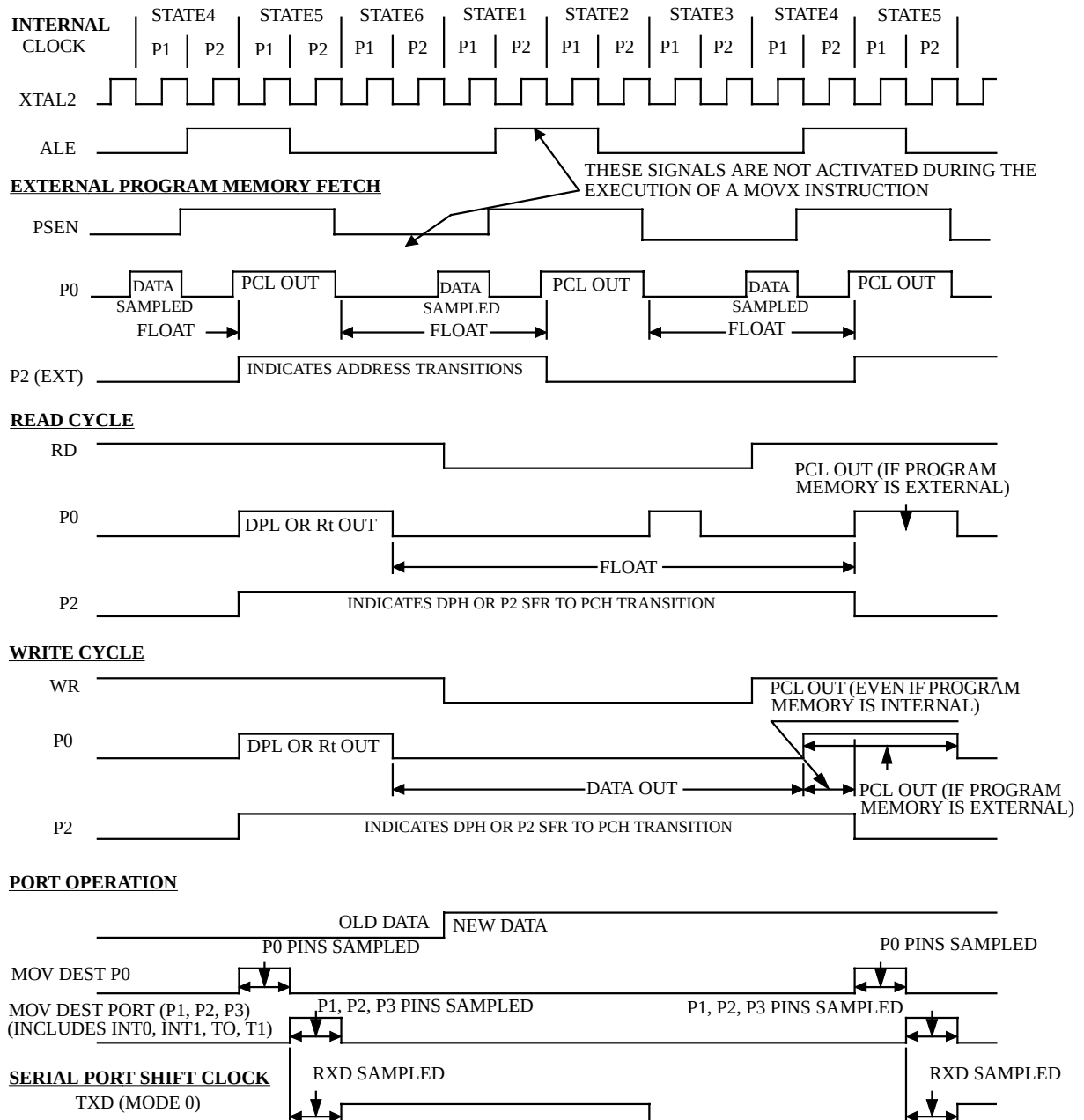
Figure 25. Clock Waveforms
