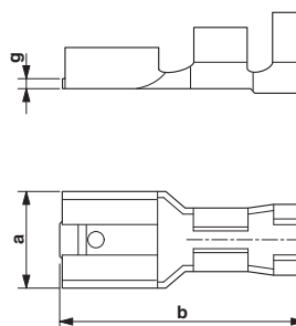
Dimensioned drawing
