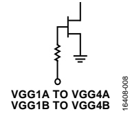
Figure 8. VGG1A to VGG4A and VGG1B to VGG4B Interface Schematic
