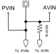
Solder Land_PVIN
