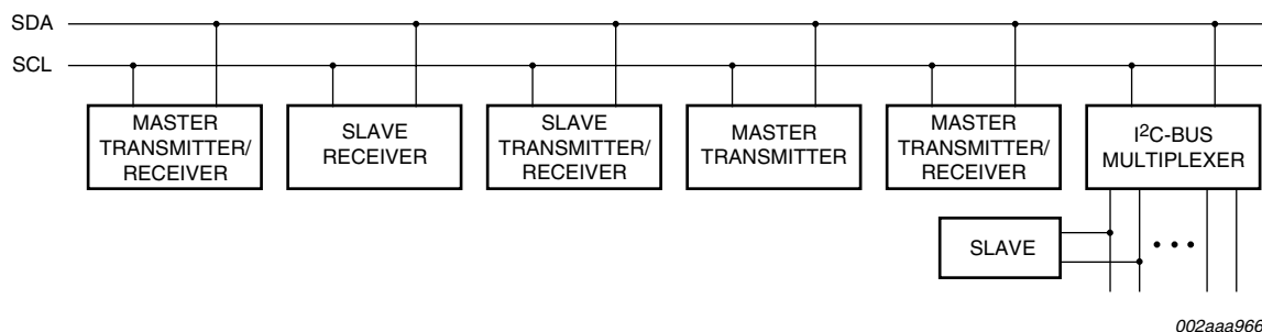
Fig 13. System configuration
