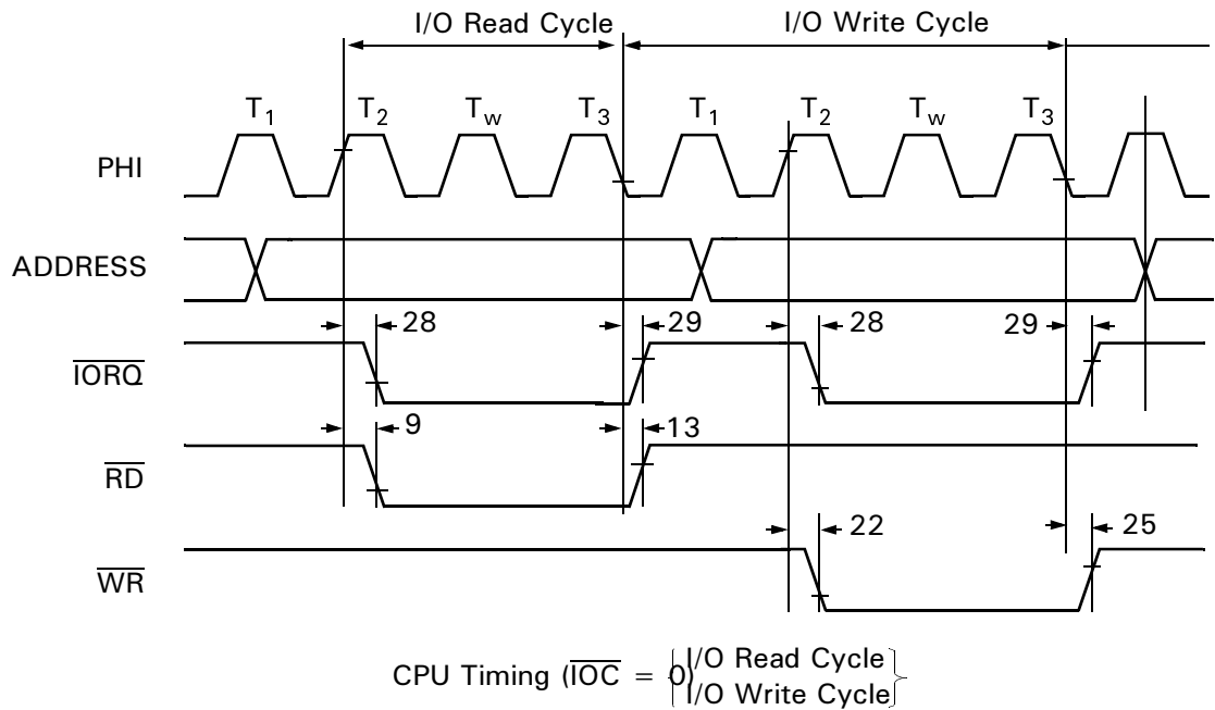
Figure 22. CPU Timing ( \overline{IO\overline{C}} = 0 ) (I/O Read Cycle, I/O Write Cycle)
