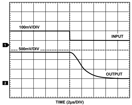
Figure 15. Fall Time
