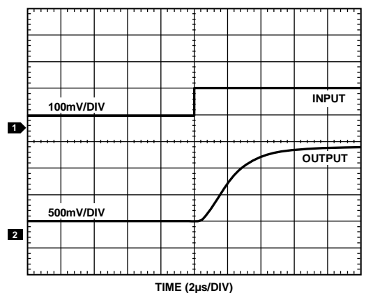
Figure 14. Rise Time
