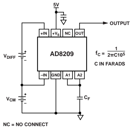
Figure 32. Single-Pole, Low-Pass Filter Using the Internal 100 k \Omega Resistor
