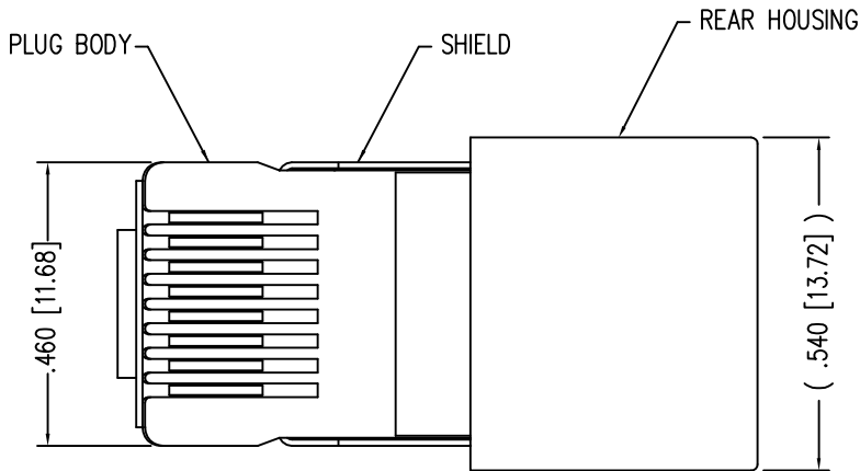
( SHOWN ASSEMBLED )
