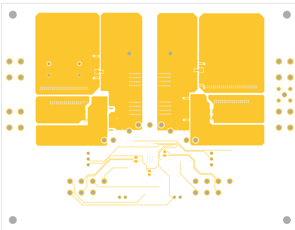
Figure 11. Bottom Layer
