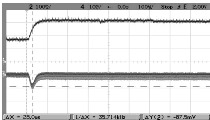
Step Load Transient Response (Vin=12V, Vout=2.5V, Cload=0, Iout=3A to 6A)
