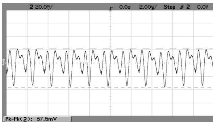
Step Load Transient Response (Vin=12V, Vout=2.5V, Cload=0, Iout=6A to 3A)
