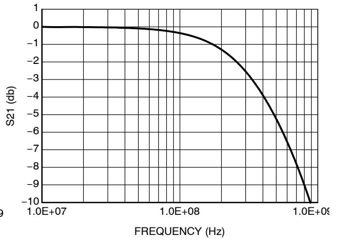
Figure 10. RF Insertion Loss
