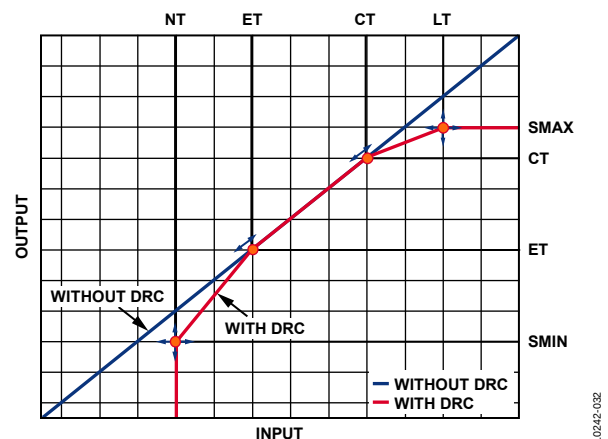
Figure 25. DRC Compression Curve: Log-to-Log Representation of the DRC Output Level vs. Input Level
