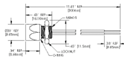
FEMALE RECEPTACLE (ACCOMMODATES THREADED MALE CORDSETS ONLY)
