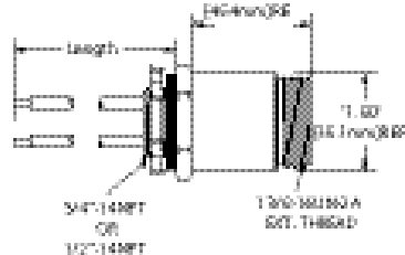
MALE RECEPTACLE
