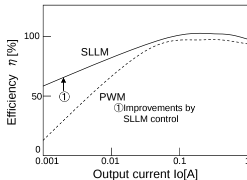
Figure.26 Efficiency characteristics
