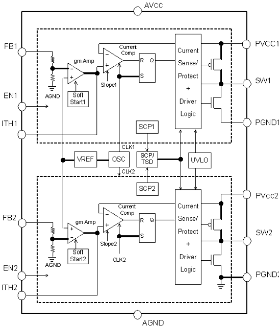
Figure.3 Block Diagram
