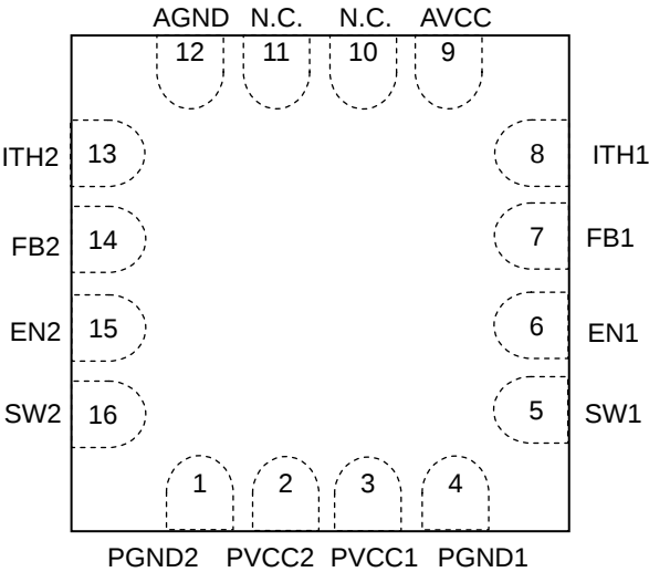
Figure.2 Pin ConFigureuration
