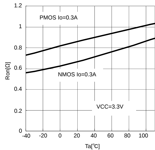
Figure.12 T_a - R_{ONN} , R_{ONP}
