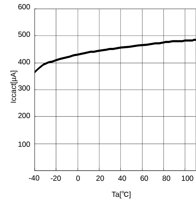
Figure.14 T_a - I_{CC}
