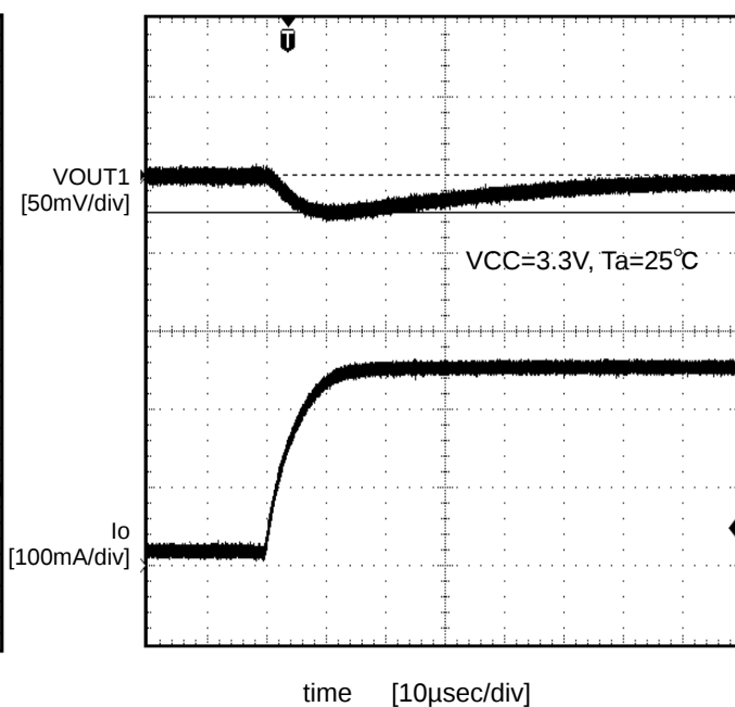
Figure.21 VOUT1 Transient response (Io=10mA→0.25A)
