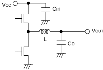
Figure.35 Input capacitor
