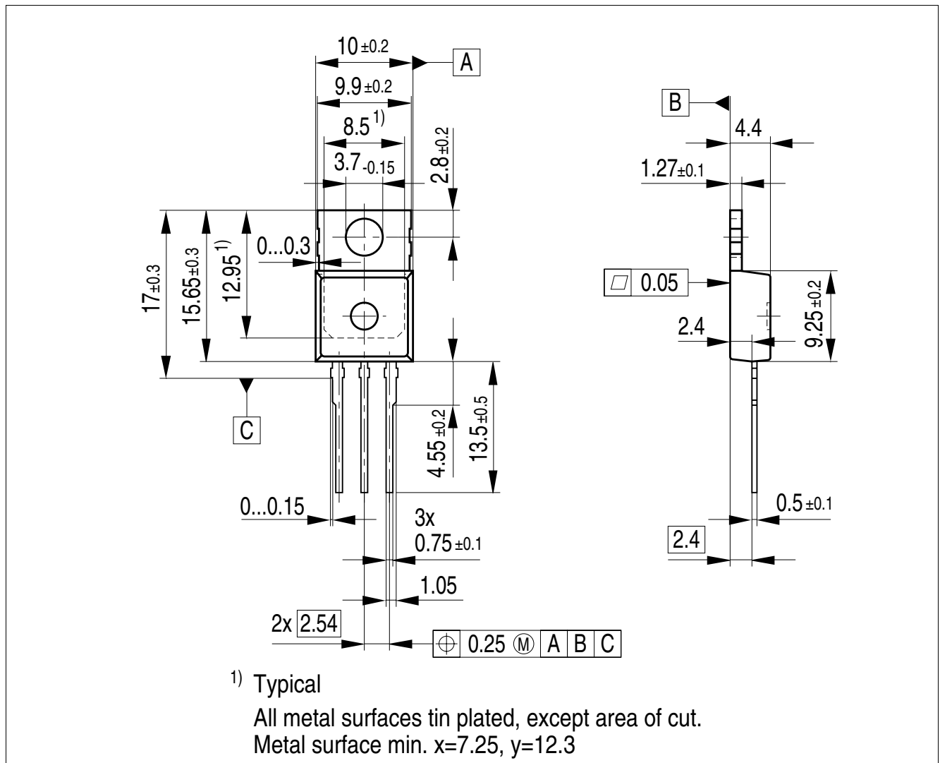
Figure 5 PG-TO220-3
