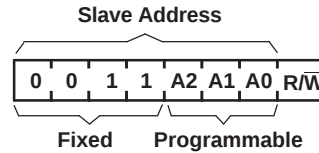
Figure 4. PCA9557 Address
