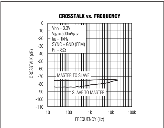
Figure 8. Master-Slave Crosstalk
