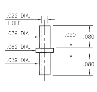
2115-2-00-XX-00-00-07-0 Swage mount in .043 hole For .062 thick board
