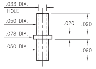
2326-2-00-XX-00-00-07-0 Swage mount in .055 hole for .062 thick board
