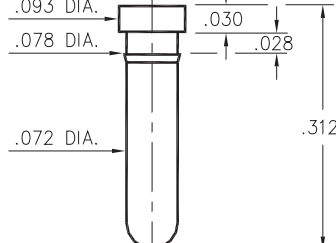
8836-0-00-XX-00-00-03-0 Press-fit in .075 mounting hole
