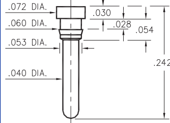
8835-0-00-XX-00-00-03-0 Press-fit in .057 mounting hole
