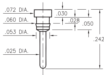
8831-0-00-XX-00-00-03-0 Press-fit in .057 mounting hole
