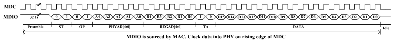
Figure 4. Write Cycle
