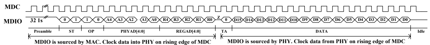
Figure 3. Read Cycle
