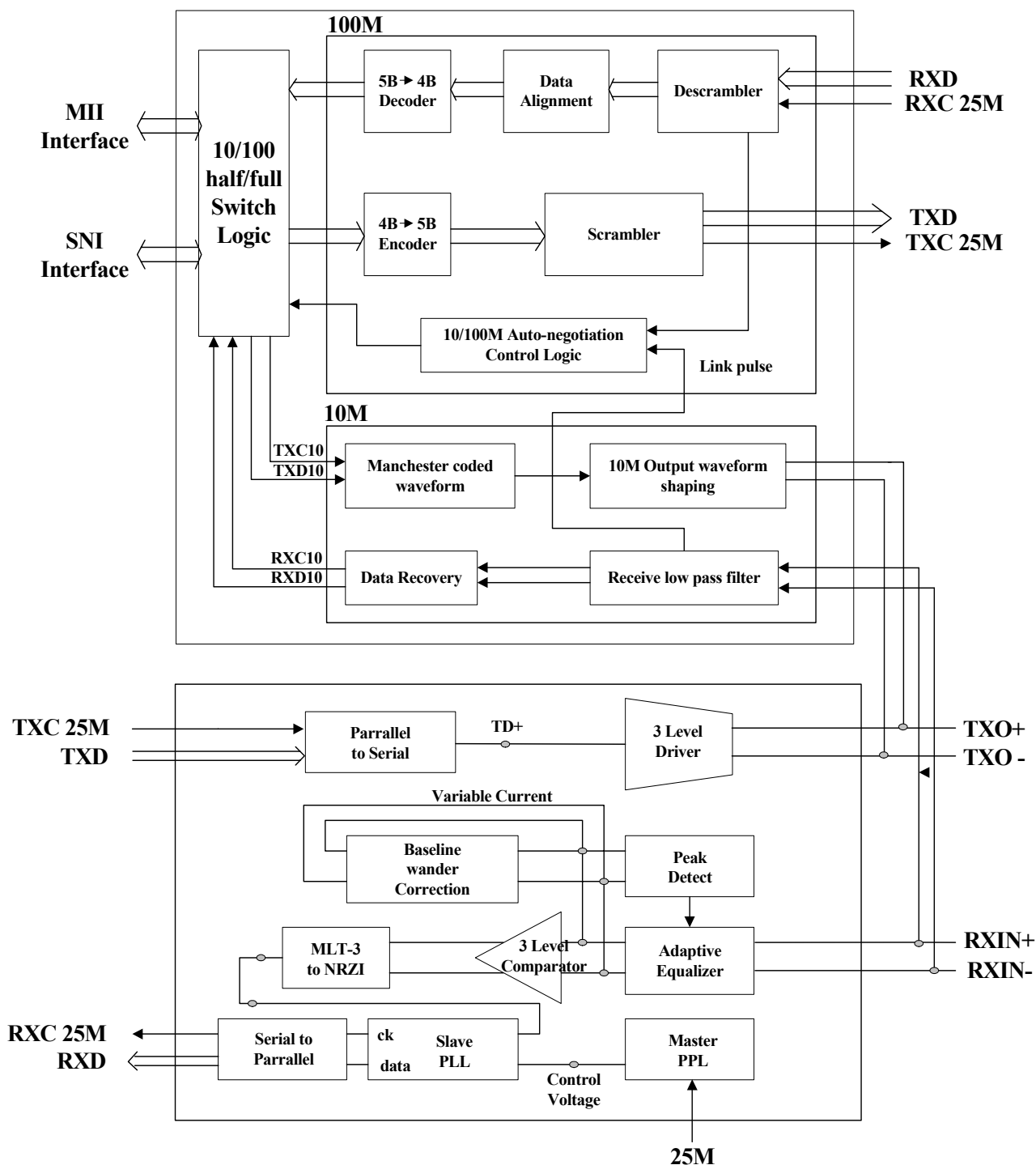
Figure 1. Block Diagram
