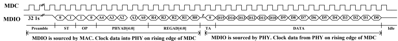
Figure 3. Read Cycle
