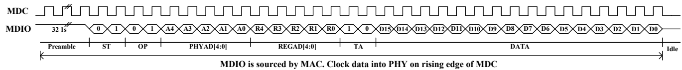
Figure 4. Write Cycle
