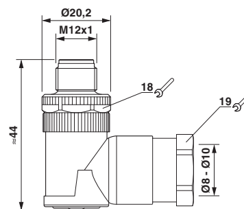
Dimensional drawing
