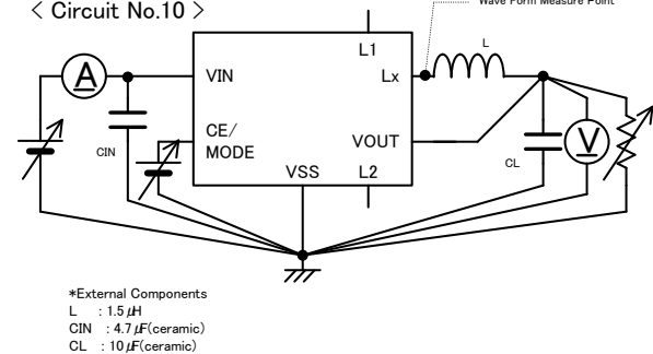
< Circuit No.10 >
