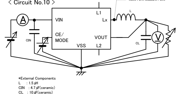
< Circuit No.10 >
