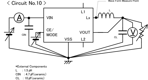
< Circuit No.10 >
