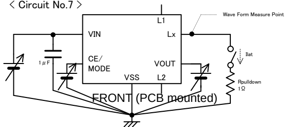
< Circuit No.7 >
