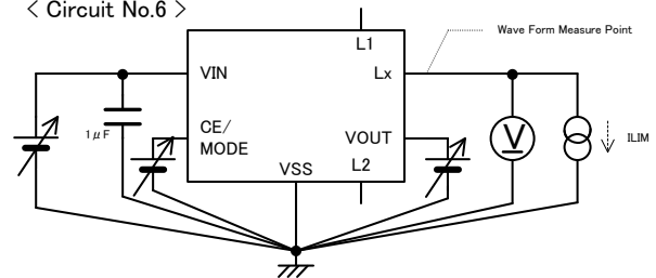
< Circuit No.6 >
