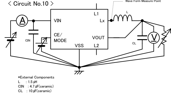
< Circuit No.10 >
