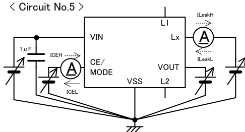
< Circuit No.5 >
