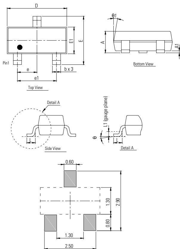
Recommended soldering pad layout (unit :mm) Drawing# : H01-B
