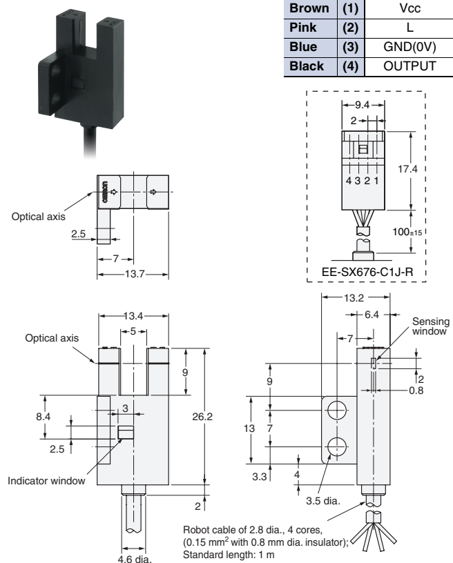
Terminal Arrangement
