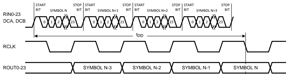
Figure 12. Deserializer Delay
