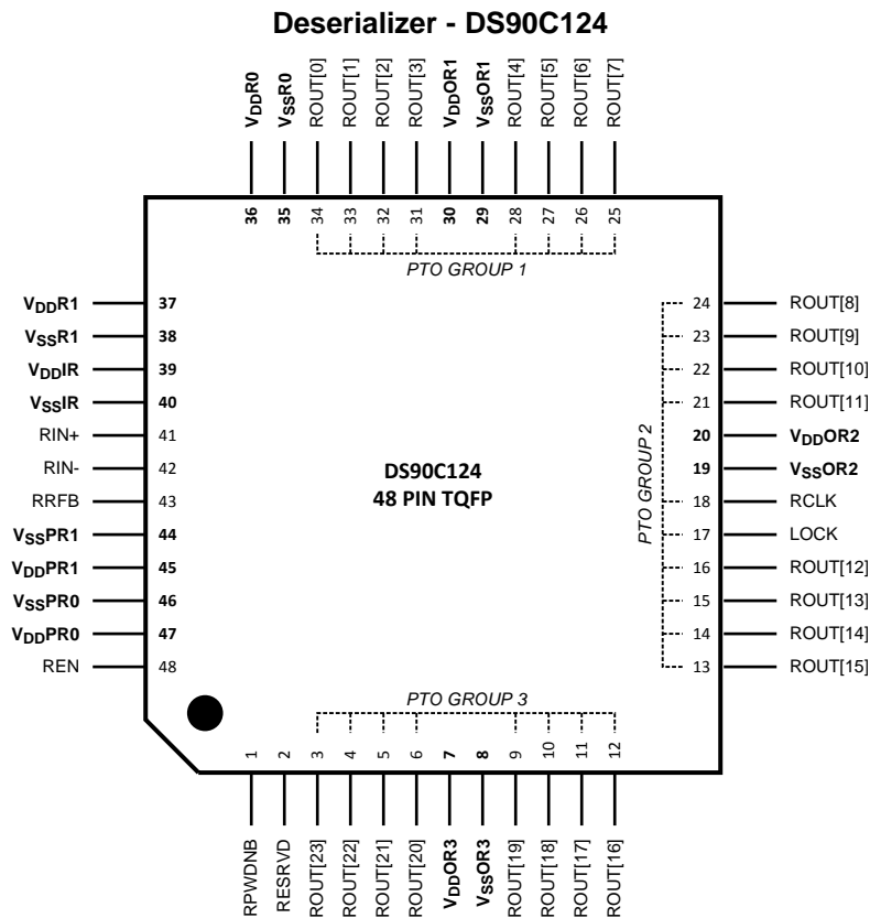
Figure 18. TOP VIEW
