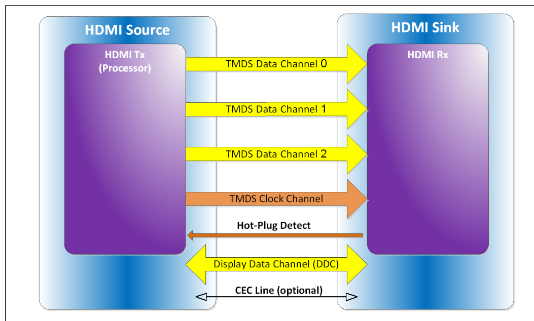
Figure 2-8. HDMI* Overview
