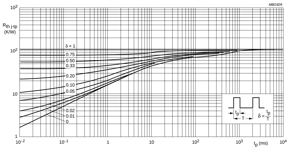
Fig.2 Thermal resistance from junction to tie-point with a lead length of 4 mm.
